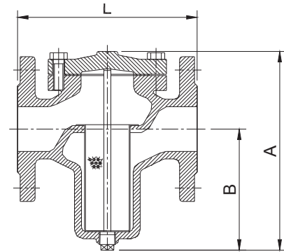
DN 50
