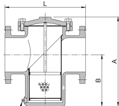
DN 50
