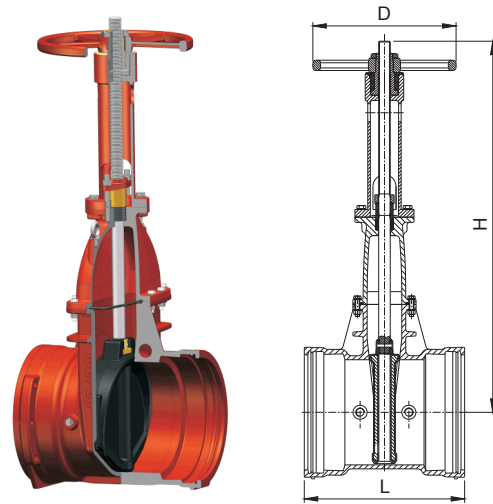
FIG. F0118-250/200, FL x PO, 14" - 16" FIG. F0188-250/200, PO x PO, 14" - 16"
