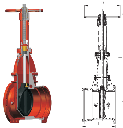
FIG. F0118-300, FL x PO, 4" - 12" FIG. F0188-300, PO x PO, 4" - 12"
